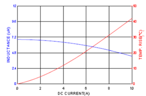
HMPL0605S-6R8
