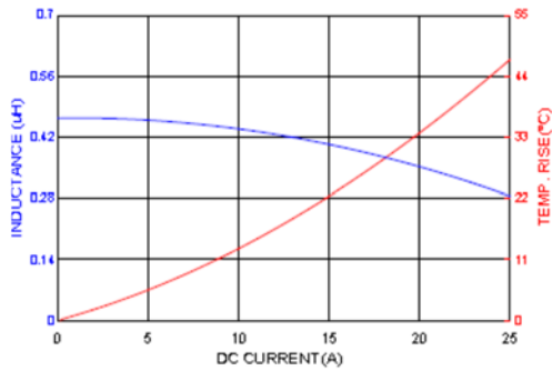
HMPL0605S-R47
