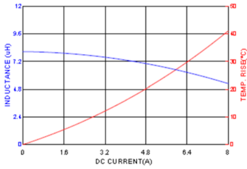
HMPL0605S-8R2
